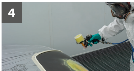
4 Apply etch primer on any bare metal areas using 3M™ Accuspray™ Gun and 1.4mm nozzle.
